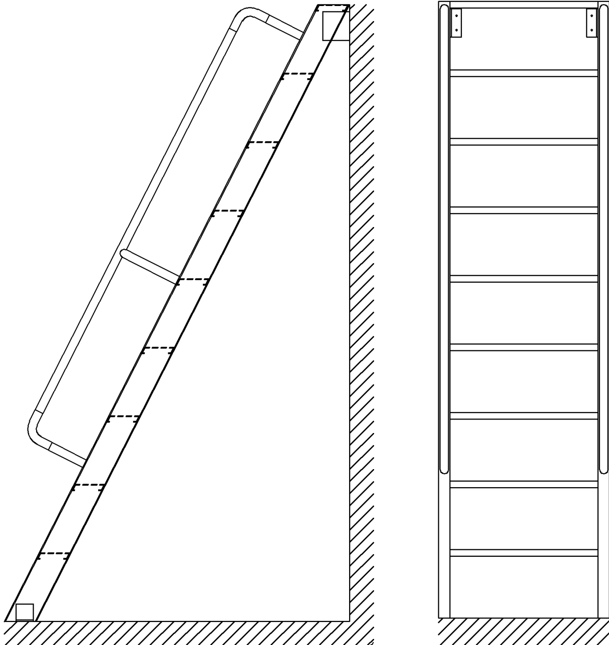
Figure 1- SHIP'S LADDER/INDUSTRIAL STAIRS
